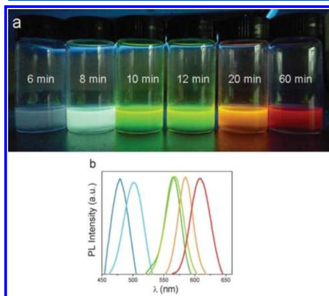
Figure 74. (a) Photographs of a series of RGO–CdSe NPs composite dispersions prepared with different reaction times under UV light irradiation of 365 nm and (b) fluorescence spectra of a series of RGO–CdSe NPs composites prepared after different reaction times. Reprinted with permission from ref 372. Copyright 2011 Royal Society of Chemistry.
