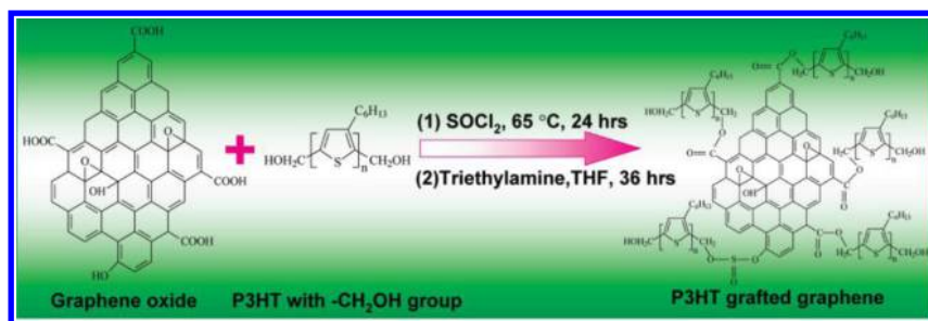
Figure 13. The reaction between GO and \text{CH}_2\text{OH} -terminated P3HT chains through an esterification reaction. Reprinted with permission from ref 104. Copyright 2010 American Chemical Society.
