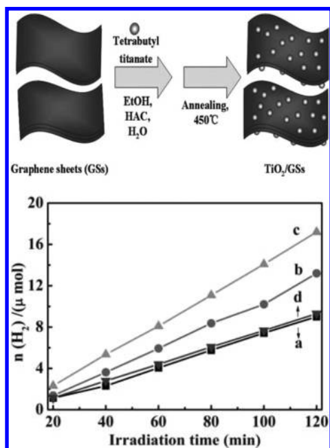
Figure 63. (top) Synthetic procedure for the preparation of RGO/TiO 2 composites. (bottom) Reaction time profiles of H 2 evolution under UV-vis irradiation over the photocatalysts: (a) TiO 2 P25 and (b) 1%, (c) 5%, and (d) 10% GO-TiO 2 . Reprinted with permission from ref 351. Copyright 2010 Royal Society of Chemistry.
