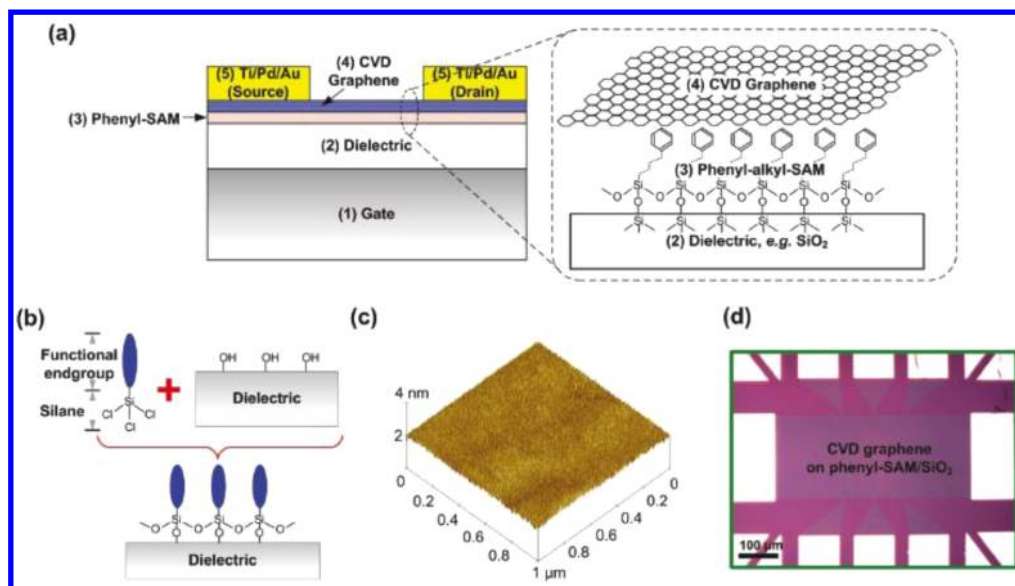
Figure 81. (a) A general bottom-gated graphene FET structure with phenyl-SAM interface engineering. (b) Illustration of chemical bonding of the organosilane SAM to the hydroxyl group-enriched dielectric surface. (c) AFM image of a spin-coated ultrasmooth phenyl-SAM with surface roughness of 0.1–0.2 nm in rms. (d) Microscopy image of a large-area, uniform CVD graphene as patterned to various shapes on a phenyl-SAM engineered silicon oxide wafer. Reprinted with permission from ref 390. Copyright 2011 American Chemical Society.
