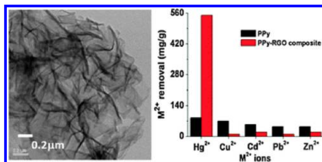
Figure 98. TEM image of graphene functionalized with polypyrrole (left) and selective adsorption of mercury from water (right). Reprinted with permission from ref 422. Copyright 2011 Royal Society of Chemistry.
