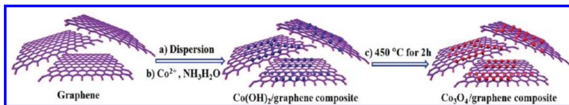
Figure 61. Schematic representation of the formation of the RGO/Co 3 O 4 composite: (a) dispersion of RGO in isopropyl alcohol/water solution, (b) formation of RGO/Co(OH) 2 composite, and (c) formation of RGO/Co 3 O 4 composite by calcination. Reprinted with permission from ref 343. Copyright 2010 American Chemical Society.
