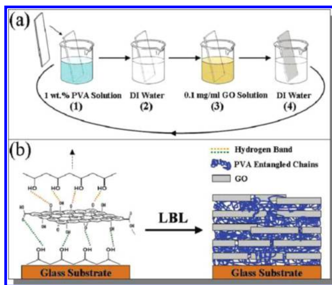
Figure 89. (a) Schematic representation of the layer by layer deposition procedure and (b) the assembly process of PVA/GO: (left) the interaction of a GO layer and PVA chains and (right) the internal architecture of PVA/GO. Reprinted with permission from ref 405. Copyright 2010 American Chemical Society.
