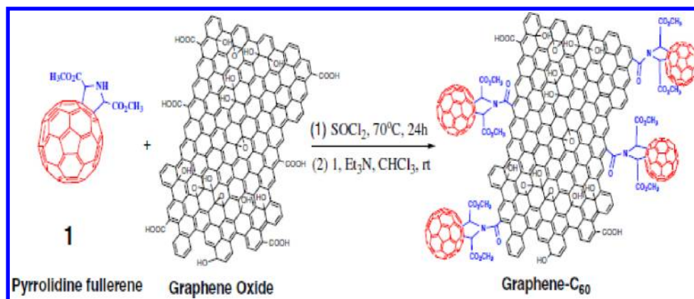
Figure 21. Representation of the formation of the C 60 -GO composite. Reprinted with permission from ref 132. Copyright 2008 Elsevier.
