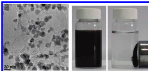
Figure 69. (left) Magnetite NPs immobilized on GO nanosheets and (right) RGO/Fe 3 O 4 removal from the water using an external magnetic force. Reprinted with permission from ref 30. Copyright 2010 American Chemical Society.
