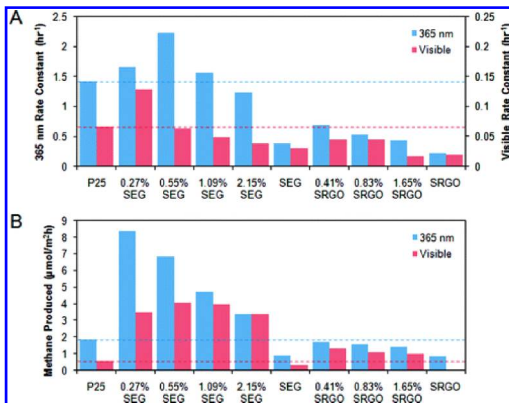
Figure 100. Photocatalytic activity of SEG–P25 and SRGO–P25 nanocomposites. (A) Pseudofirst-order CH 3 CHO photo-oxidation rate constants for SEG–P25 and SRGO–P25 nanocomposites under ultraviolet (365 nm) and visible illumination. (B) CO 2 photoreduction for SEG–P25 and SRGO–P25 nanocomposites under ultraviolet (365 nm) and visible illumination. Reprinted with permission from ref 429. Copyright 2011 American Chemical Society.
