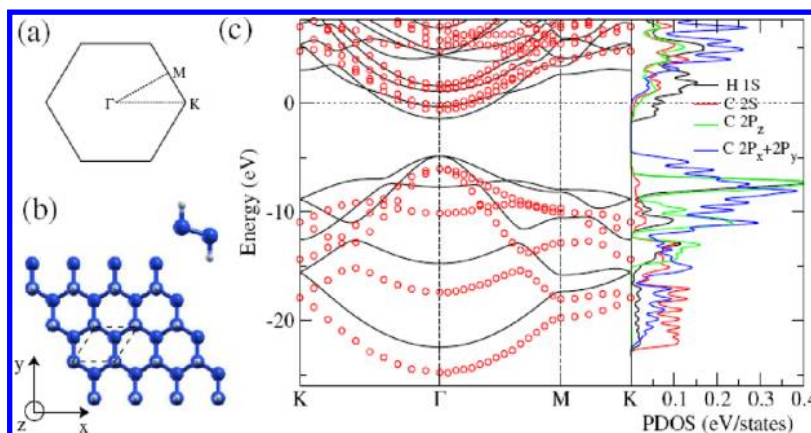
Figure 33. (a) First Brillouin zone and (b) unit cell and bases of graphane in the chair conformation. Blue and white balls represent carbon and hydrogen atoms, respectively. (c) Band structure in local-density approximation (LDA, full line) and GW approximation (circles) and projected density of states of graphane. The zero level indicates the vacuum level position. Reprinted with permission from ref 162. Copyright 2010 American Physical Society.
