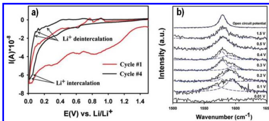
Figure 87. (a) First and fourth cyclic voltammograms of the Ni/FLG electrode in polymer electrolyte and (b) in situ Raman spectra of the Ni/FLG electrode at selected potentials during electrochemical lithiation. Reprinted with permission from ref 398a. Copyright 2010 American Chemical Society.
