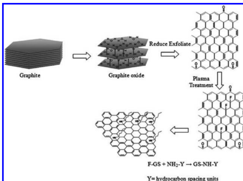
Figure 24. Preparation of butylamine-functionalized RGO nanoplatelets. Reprinted with permission from ref 138. Copyright 2009 American Chemical Society.
