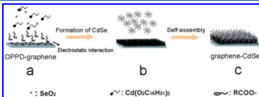
Figure 73. Schematic representation of the formation of RGO/CdSe NP composite. Reprinted with permission from ref 372. Copyright 2011 Royal Society of Chemistry.
