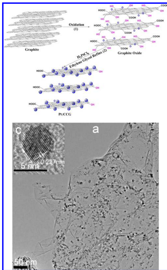
Figure 54. (Top) Schematic of formation of RGO/Pt and (bottom) TEM images of dispersion of Pt nanoparticles on graphenes. Reprinted with permission from ref 328. Copyright 2010 Royal Society of Chemistry.
