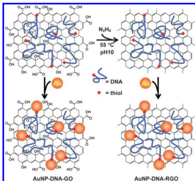
Figure 43. DNA coating and aqueous dispersion of GO and RGO, which were then used as two-dimensional bio–nano-interfaces for homogeneous assembly of metal–carbon heteronanostructures. Reprinted with permission from ref 275. Copyright 2010 Royal Society Chemistry.
