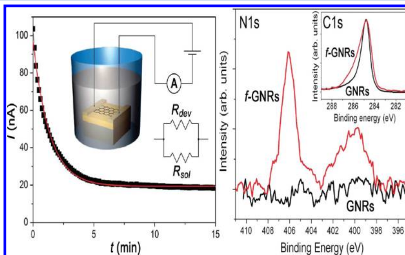
Figure 2. Time dependence of current I : (left) Scheme of the experiment shows the device consisted of two parallel resistances derived from the graphene and the solution, and (right) N1s and C1s XPS spectra of GNRs before and after the functionalization (f-GNRs). Reprinted with permission from ref 64. Copyright 2010 American Chemical Society.
