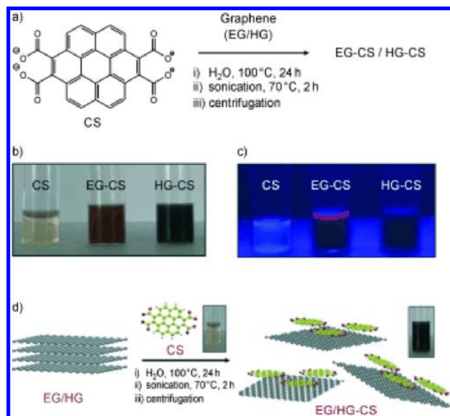
Figure 47. (a) Synthetic scheme for the preparation of graphene–coronene composites. (b) Photographs of the aqueous solutions of CS, EG–CS, and HG–CS and (c) corresponding images under UV/vis illumination. (d) Schematic illustration of the exfoliation of few-layer graphene with CS to yield monolayer graphene–CS composites. Reprinted with permission from ref 291. Copyright 2010 Wiley.
