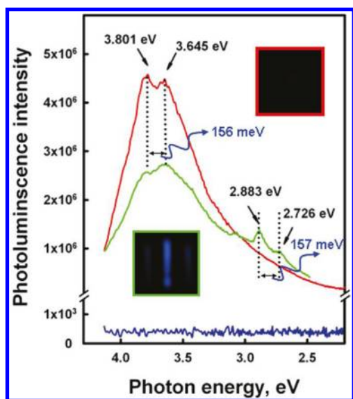
Figure 37. Photoluminescence emission spectra at room temperature (excitation at 290 nm, 4.275 eV) of graphene (blue) and fluorographene (green, 1 day fluorination; red, 5 days). The difference between the main emission peaks is 156 meV ( 1260\text{ cm}^{-1} ); this corresponds to the energy of a C–F vibration. The blue emission (at 2.88 eV) lasts ca. 30 s after excitation, and its exact origin is uncertain. Reprinted with permission from ref 175. Copyright 2011 American Chemical Society.
