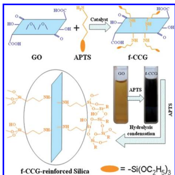
Figure 25. Illustration of the reaction between GO and APTS and incorporation of Si- f -GO nanoplatelets into the silica matrix. R = -\text{OH} or -\text{CH}_2(\text{CH}_2)_2\text{NH}_2 . Reprinted with permission from ref 143. Copyright 2009 Royal Society of Chemistry.
