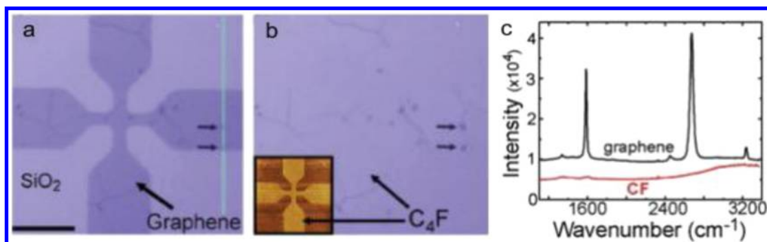
Figure 36. One side fluorination (one side fluorinated graphene C_4F , panel b) changes the optical properties of graphene (panel a). Raman signal of stoichiometric fluorographene (CF, panel c) disappears. The spectra of graphene and fluorographene are offset for clarity. Reprinted with permission from ref 169. Copyright 2010 American Chemical Society.
