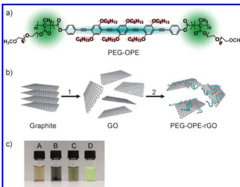
Figure 49. (a) Chemical structure of PEG-OPE. (b) The synthesis of PEG-OPE-rGO in H 2 O. Step 1, oxidation of graphite yields single-layer GO nanoplatelets. Step 2, Chemical reduction of GO with hydrazine in the presence of PEG-OPE produces a stable aqueous suspension of PEG-OPE-rGO. (c) Photograph of (A) GO and (B) RGO in water and (C) PEG-OPE-rGO and (D) PEG-OPE in methanol. Reprinted with permission from ref 305. Copyright 2010 Wiley.
