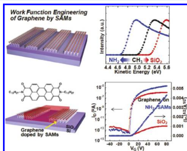
Figure 82. Transferred monolayer graphene on patterned self-assembled monolayer (SAM)-modified \text{SiO}_2 substrate (top left). UV photoemission spectra of the graphene films on different SAM-modified substrates show work function changes (top right). Chemical structure of N,N' -ditridenyl-3,4,9,10-perylene-tetracarboxylic diimide (PTCDI-C13) and schematic FET structure using PTCDI-C13 as an active layer and graphene as source/drain electrodes (bottom left). Transfer characteristics of PTCDI-C13 FETs with graphene electrodes on different SAM-modified \text{SiO}_2 's (bottom right). Reprinted with permission from ref 46. Copyright 2011 American Chemical Society.
