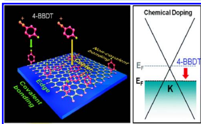
Figure 46. Noncovalent functionalization occurs on the basal plane of defect-free graphene, as opposed to covalent bonding formed on the edge of the graphene. Doping induces modulation of the Fermi level of graphene. Reprinted with permission from ref 288. Copyright 2010 American Chemical Society.
