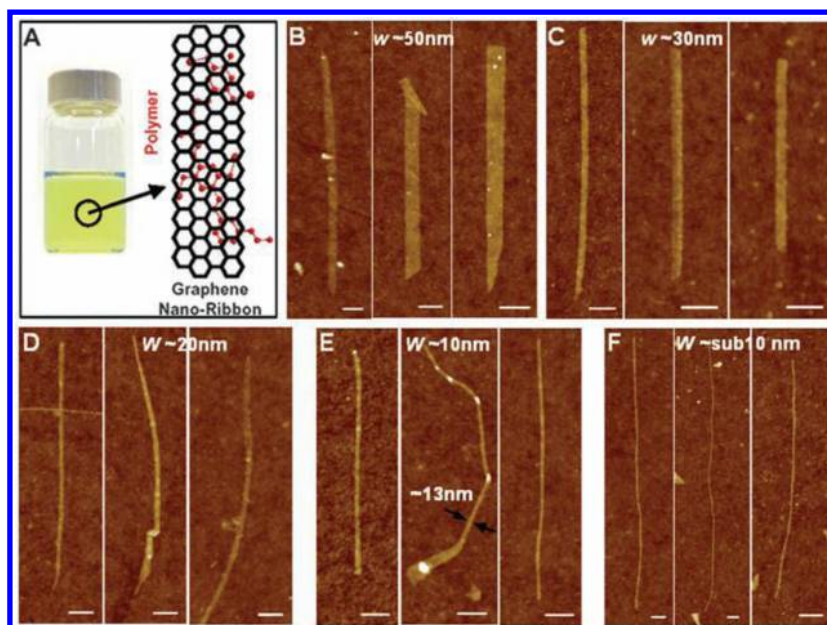
Figure 48. (A) (left) Photograph of a polymer PmPV/DCE solution with GNRs stably suspended in the solution and (right) schematic drawing of a graphene nanoribbon with two units of a PmPV polymer chain adsorbed on top of the graphene via \pi stacking. (B–F) Chemically derived graphene nanoribbons down to sub-10-nm width. Reprinted with permission from ref 59. Copyright 2008 American Association for the Advancement of Science.
