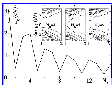
Figure 35. Dependence of band gap ( E_g in eV) of armchair nanoroads on nanoroad width ( N_a ). The insets show band structures of armchair nanoroads of width ( N_a ) 4, 5, and 6. Reprinted with permission from ref 167. Copyright 2009 American Chemical Society.
