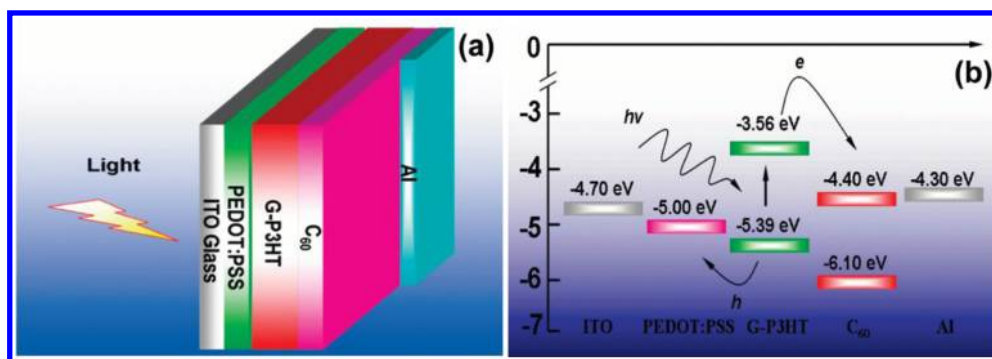
Figure 14. (a) Schematic and (b) energy level diagram of a ITO/PEDOT:PSS/GO–P3HT/C60/Al photovoltaic device. Reprinted with permission from ref 104. Copyright 2010 American Chemical Society.
