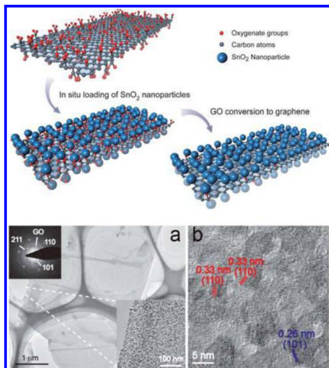
Figure 59. (top) Schematic representation of the formation of the GO/SnO 2 composite. (bottom) (a) TEM image of SnO 2 NPs loaded on GO with corresponding SAED pattern and (b) HRTEM image of the SnO 2 -GO composite. Reprinted with permission from ref 339. Copyright 2010 Royal Society of Chemistry.
