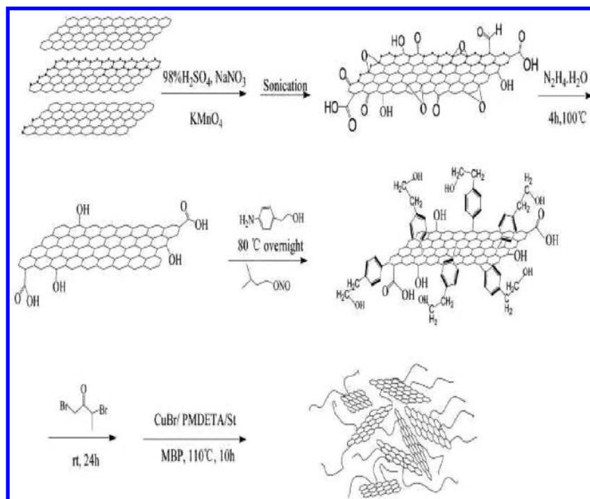
Figure 3. The attachment of aryl groups on graphene nanosheets and the formation of polystyrene chains grafted on graphene nanosheets. Reprinted with permission from ref 71. Copyright 2009 Royal Society of Chemistry.
