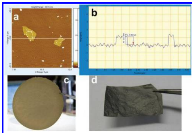
Figure 75. (a) AFM image of GO and (b) related height profile, (c) Si/GO composite paper, and (d) Si/RGO composite paper obtained by reduction of Si/GO. Reprinted with permission from ref 373. Copyright 2010 Royal Society of Chemistry.
