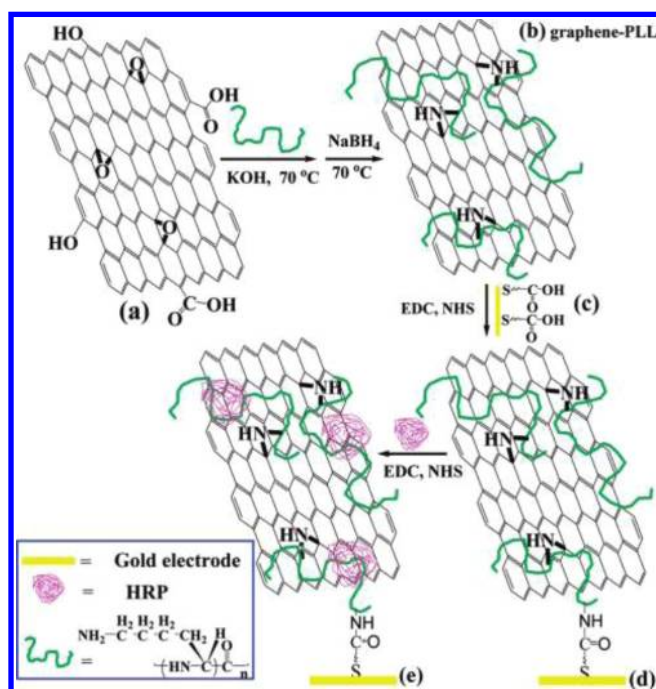
Figure 18. Schematic representation of the formation of the PLL/RGO-horseshoe peroxidase and its subsequent deposition on a gold electrode. Reprinted with permission from ref 112. Copyright 2009 American Chemical Society.
