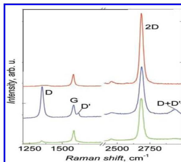
Figure 32. Raman spectra of pristine graphene (red), graphane (blue), and graphane after annealing (green). In the Raman spectrum of graphane the D defect peak becomes active, as well as the appearance of D' and D+D' peaks. Reprinted with permission from ref 42. Copyright 2009 American Association for the Advancement of Science.
