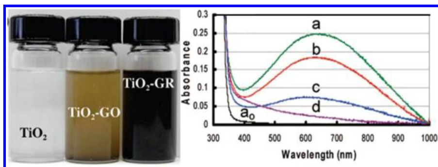
Figure 64. (left) The change in color of a suspension of GO/TiO 2 before and after UV irradiation. A suspension of TiO 2 NPs is also shown for comparison. (right) Absorption spectra of UV-irradiated TiO 2 suspension (a) before and (b–d) after the addition of GO suspensions: (b) 50, (c) 150, and (d) 300 \mu\text{g} of GO ( a 0 corresponds to the TiO 2 suspension prior to UV irradiation). Reprinted with permission from ref 18. Copyright 2008 American Chemical Society.
