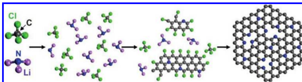
Figure 79. A possible mechanism for the solvothermal synthesis of N-doped graphene. Reprinted with permission from ref 381. Copyright 2011 American Chemical Society.
