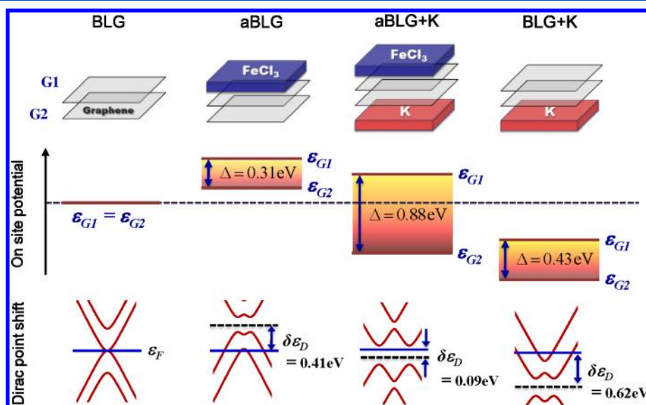
Figure 84. Schematic models of the bilayer graphene (BLG), the BLG doped with FeCl 3 (aBLG) composite system, the BLG dual-doped with FeCl 3 and K (aBLG+K), and the BLG doped with K (BLG+K) (top), tight binding parameters for the onsite potential difference ( \Delta ) obtained by DFT calculation (center), and band structures calculated by tight binding method and the Dirac point shifts ( \delta\epsilon_D ) obtained by DFT calculation (bottom). Reprinted with permission from ref 394. Copyright 2011 American Chemical Society.
