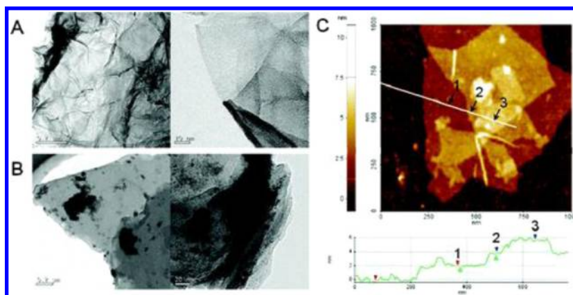
Figure 50. TEM images of chemically converted graphene nanoplatelets (a) in the presence of and (b) in the absence of ILP and (c) tapping mode AFM image of the ILP-G processed from organic suspension and height profiles across the ILP-G sheets indicating a thickness of \sim 1.9 nm. Reprinted with permission from ref 306. Copyright 2010 American Chemical Society.
