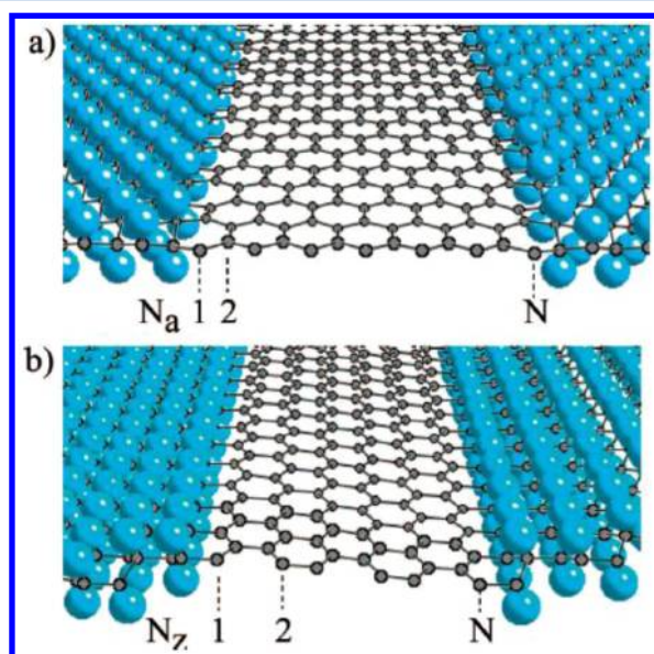
Figure 34. Structures of (a) armchair and (b) zigzag graphene nanoroads in graphane. N_a denotes width of sp^2 carbon lines in armchair and N_z in zigzag roads. Reprinted with permission from ref 167. Copyright 2009 American Chemical Society.
