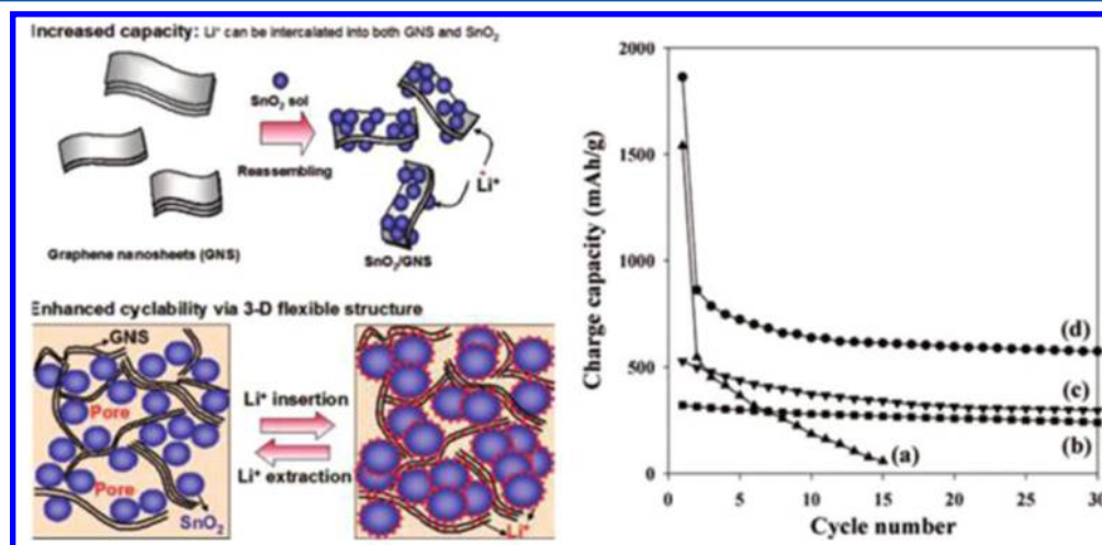
Figure 58. (left) Schematic representation of the formation of RGO/SnO 2 and its use in Li ion batteries and (right) cyclic performances for (a) SnO 2 nanoparticles, (b) graphite, (c) RGO nanoplatelets, and (d) RGO/SnO 2 . Reprinted with permission from ref 330. Copyright 2008 American Chemical Society.
