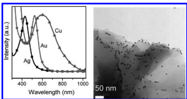
Figure 57. (Left) UV-vis absorption spectra of Ag, Au and Cu NPs deposited on RGO and (right) TEM image of the RGO nanoplatelet with Au NPs deposited on the surface. Reprinted with permission from ref 329. Copyright 2009 Royal Society of Chemistry.
