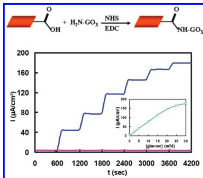
Figure 20. (top) Immobilization of glucose oxidase (H 2 N-GO x ) onto GO nanoplatelets. (bottom) Typical amperometric response of the GO x -GO electrode (blue line) and the pristine graphene electrode (pink line). Inset shows calibration curve obtained for glucose determination at 0.4 V vs Ag/AgCl. Reprinted with permission from ref 131. Copyright 2010 American Chemical Society.
