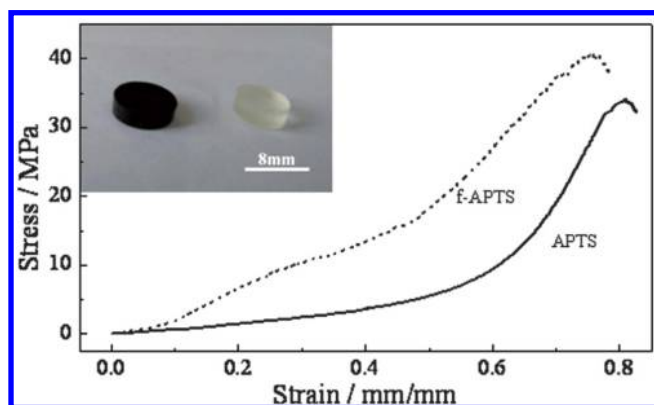
Figure 26. Stress–strain plots of neat APTS monolith (solid) and Si- f -GO reinforced APTS monolith (dotted). Inset: photographs of monolith disks for the compressive tests. From left to right: Si- f -GO reinforced APTS monolith and neat APTS monolith. Reprinted with permission from ref 143. Copyright 2009 Royal Society of Chemistry.
