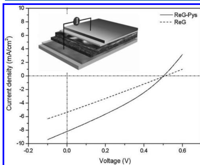
Figure 40. Current density vs voltage ( I – V ) curves of P3HT/PCBM heterojunction solar cells with 10 nm thick thermally reduced ReG and ReG–PyS films as the transparent electrodes, respectively. Inset is a schematic illustration of the solar cell; the five layers from top to bottom are Al, ZnO, a blend of P3HT and PCMB, PEDOT:PSS, graphene, and quartz, respectively. Reprinted with permission from ref 91. Copyright 2009 Wiley.
