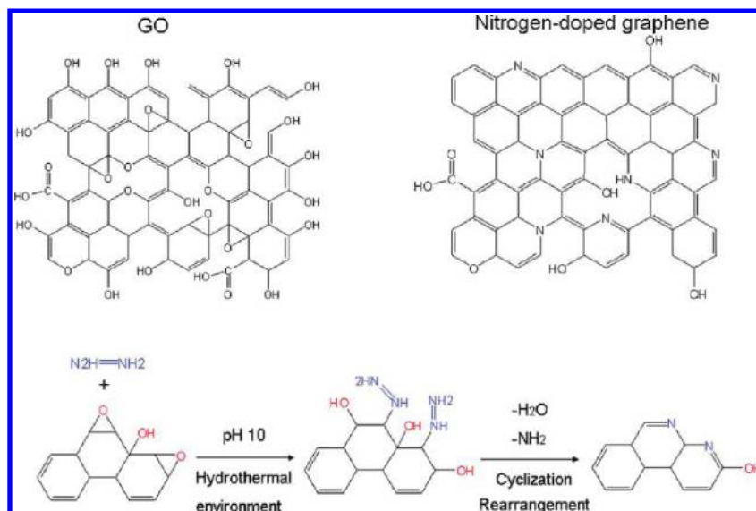
Figure 78. Schematic structure of GO and N-doped GO produced by hydrothermal reduction. Reprinted with permission from ref 377. Copyright 2010 American Chemical Society.
