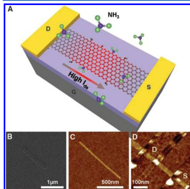
Figure 77. Electrothermal reaction of an individual GNR in \text{NH}_3 : (a) schematic representation of the device electrically annealed under \text{NH}_3 (where D is the drain, S the source, and G the gate); (b) SEM and (c) AFM images of a \sim 30 nm wide GNR and (d) AFM image of the device fabricated on the GNR. Reprinted with permission from ref 43. Copyright 2009 American Association for the Advancement of Science.
