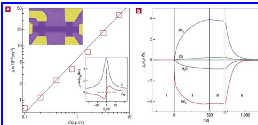
Figure 80. (a) Concentration of chemically induced charge carriers in SLG exposed to different concentrations of \text{NO}_2 and (b) changes in resistivity at zero \mathbf{B} field caused by graphene's exposure to various gases diluted to 1 ppm. Reprinted with permission from ref 384a. Copyright 2008 American Chemical Society.
