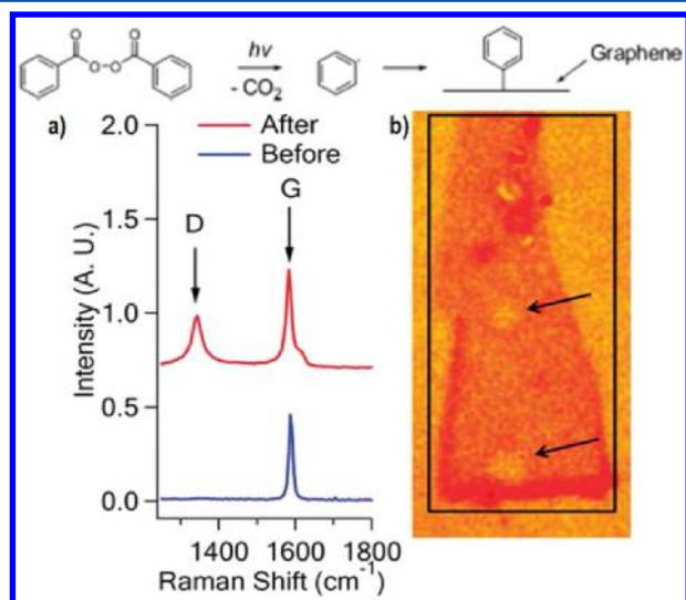
Figure 4. Schematic representation of the radical addition reaction: (a) the appearance of D band in the Raman spectrum of a single layer graphene after the photochemical reaction and (b) optical image of a functionalized single-layer graphene. The arrows indicate holes resulting from prolonged laser exposure. Reprinted with permission from ref 72. Copyright 2009 American Chemical Society.
