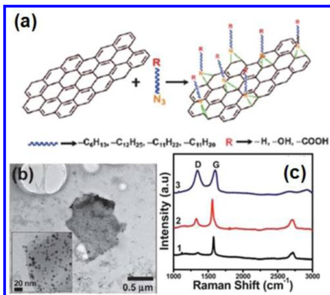
Figure 9. (a) The reaction of alkyl nitrenes with graphene sheets. (b) TEM images of the Au decorated graphene nanoplatelets after organic modification with undecanoic acid groups. (c) Raman spectra of graphene sheet before (1) and after the nitrene addition of azidoundecanoic acid in 1:1 (2) and 10:1 (3) ratios. Reprinted with permission from ref 85. Copyright 2011 Royal Society of Chemistry.
