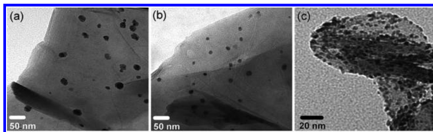
Figure 56. TEM images of RGO nanoplatelets decorated with (a) Pd, (b) Cu, and (c) CuPd NPs. Reprinted with permission from ref 329. Copyright 2009 Royal Society of Chemistry.
