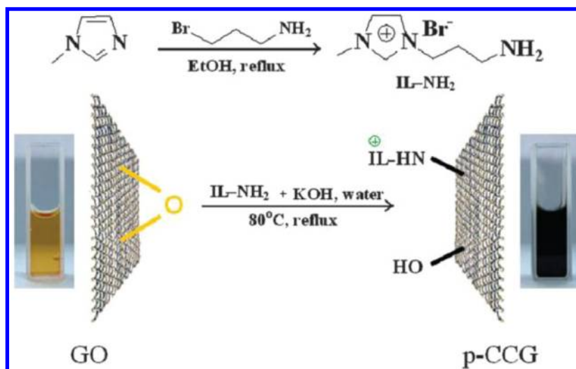
Figure 22. Illustration of the preparation of imidazolium-modified GO. Reprinted with permission from ref 135. Copyright 2009 Royal Society of Chemistry.
