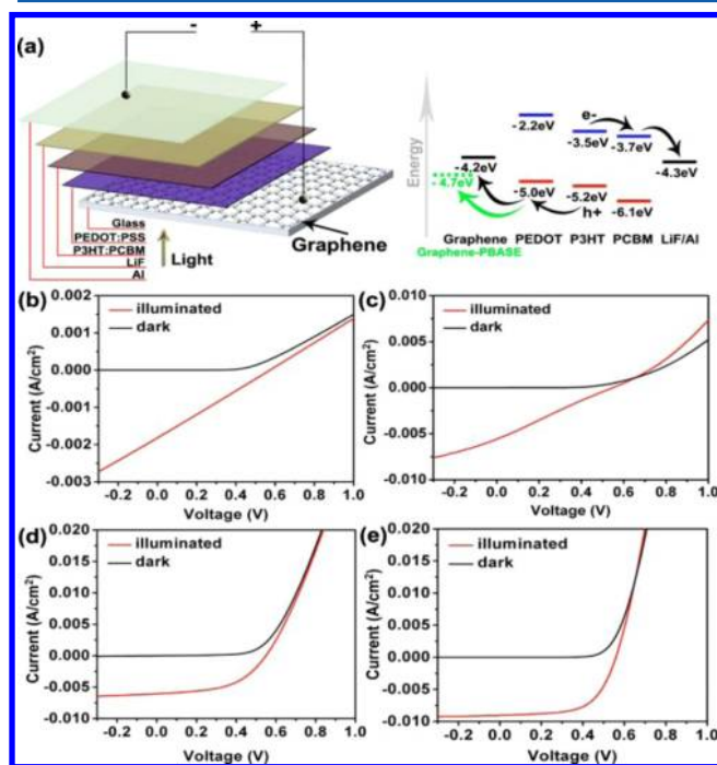
Figure 39. (a) Energy diagram of the fabricated device structure graphene/PEDOT:PSS/P3HT:PCBM/LiF/Al. (b–e) Current–voltage characteristics of the photovoltaic devices based on graphene films in the dark and under illumination: (b) pristine graphene film, (c) graphene film treated by UV light, (d) graphene film modified by PBSA, and (e) ITO anode for comparison. Reprinted with permission from ref 268. Copyright 2009 American Institute of Physics.
