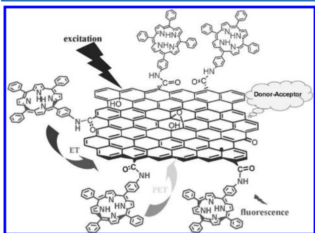
Figure 15. Schematic representation of the product of the reaction between GO and amine-functionalized porphyrin. Reprinted with permission from ref 106. Copyright 2009 Wiley.
