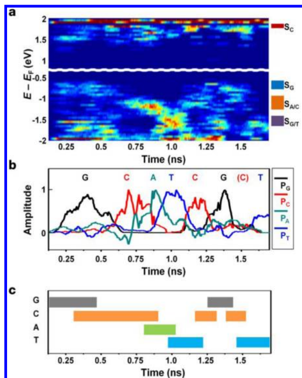
Figure 96. Simulation results of the transport property for 5'-GCATCGCT-3'. (a) Time-dependent histogram of the transmission peak positions (red (blue) denoting maximal (minimal) values). The histogram shows features of Cyt ( S_C ), Gua ( S_G ), Ade/Cyt ( S_{A/C} ), and Gua/Thy ( S_{G/T} ) corresponding to the band centered around E - E_F = E_s = 1.8, -0.65, -1.2, and -1.65 eV, respectively. The height of each right box represents the energy range of integration for S_{base} . (b) Plots of S_{base}(t) with respect to time as a ssDNA passes. The sequence GCATCGCT can be partly resolved. (c) Final base sequence obtained from the analysis of panel b and 2D TACF, C(t, t_0; \tau) analysis. Reprinted with permission from ref 37. Copyright 2011 Nature Publishing Group.
