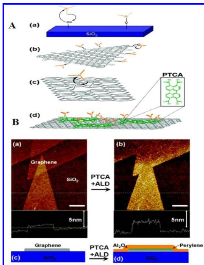
Figure 41. (A) Schematics of atomic layer deposition of aluminum oxide via trimethylaluminum (TMA) precursor on (a) bare \text{SiO}_2 substrate, (b) a single layer graphene sheet with edges, (c) graphene containing a defect site, and (d) perylene tetracarboxylic acid (PTCA)-coated graphene. PTCA selectively adheres to graphene on \text{SiO}_2 surfaces, providing binding sites for TMA deposition. Inset is a top view of the PTCA structure. (B) ALD of \text{Al}_2\text{O}_3 on PTCA-coated graphene. (a) AFM image of graphene on \text{SiO}_2 before ALD. The height of the triangular shaped graphene is \sim 1.6 nm as shown in the height profile along the dashed line. Scale bar is 500 nm. (b) AFM image of the same area as panel a after \sim 2 nm \text{Al}_2\text{O}_3 ALD deposition. The height of the triangular shaped graphene becomes 3.0 nm as shown in the height profile along the dashed line. Scale bar is 500 nm. (c,d) Schematics of graphene on \text{SiO}_2 before and after ALD. The \text{Al}_2\text{O}_3 grows uniformly on the noncovalently PTCA-coated graphene. Reprinted with permission from ref 274. Copyright 2008 American Chemical Society.
