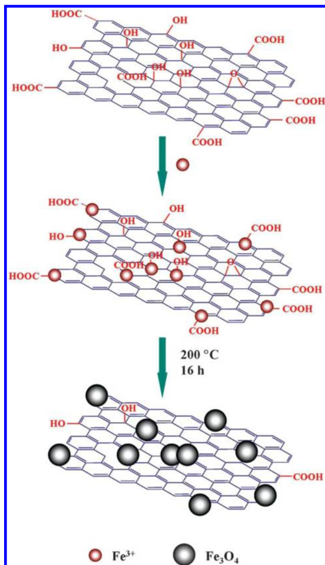
Figure 70. Deposition of magnetite nanoparticles on RGO nanosheets. Reprinted with permission from ref 362. Copyright 2010 Royal Society of Chemistry.
