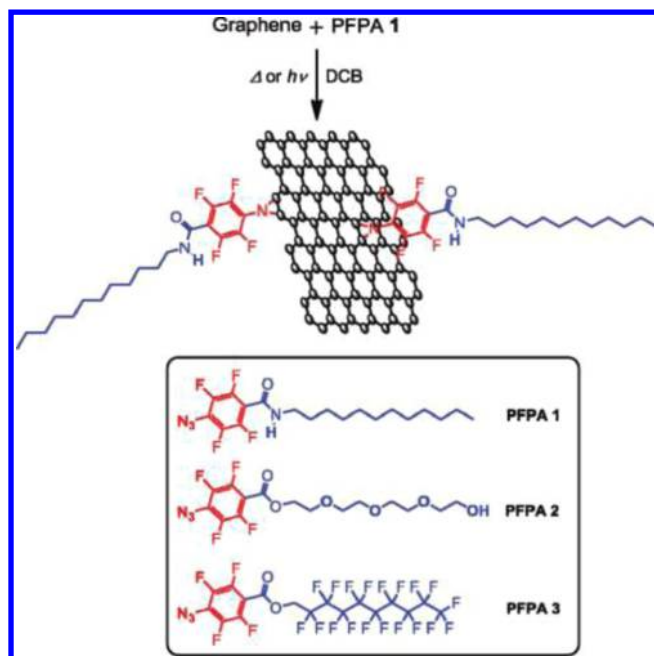
Figure 7. Functionalization of pristine graphene with PFFPA. Reprinted with permission from ref 83. Copyright 2010 American Chemical Society.
