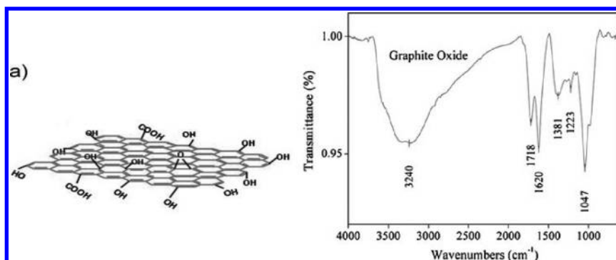
Figure 11. (left) Structure of GO and (right) its FTIR spectrum. Left panel reprinted with permission from ref 101. Copyright 2009 Wiley. Right panel reprinted with permission from ref 102; Copyright 2011 Indian Academy of Sciences.
