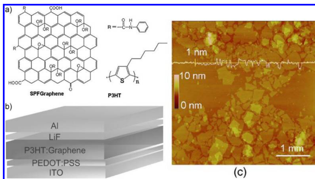
Figure 27. (a) Graphical representation of the modified graphene and P3HT, (b) schematic representation of the bulk heterojunction photovoltaic cells, and (c) an AFM image of the modified graphene. Reprinted with permission from ref 146. Copyright 2009 Wiley.
