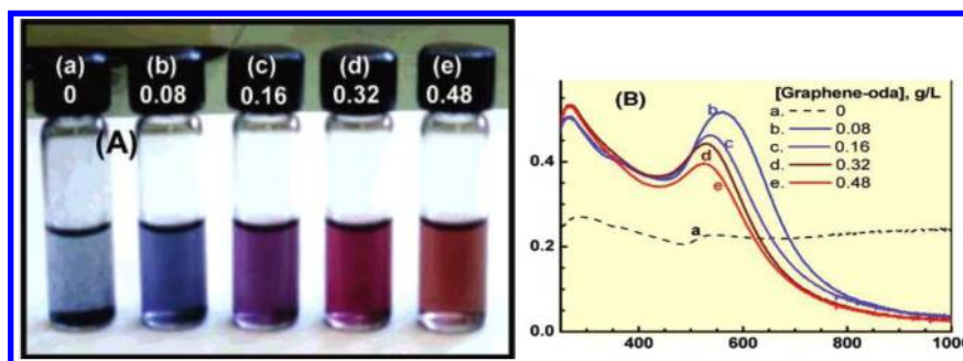
Figure 51. (Left) Photograph of several dispersions of gold nanoparticles (1 mM) in THF with different concentrations of GO–ODA (octadecylamine) and (right) the characteristic UV–vis absorption spectra of the dispersions. Reprinted with permission from ref 318. Copyright 2008 American Chemical Society.
