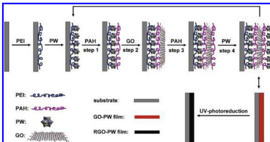
Figure 90. Schematic illustration of the LbL deposition of GO and PW clusters and the photoreduction of GO. Cationic polyelectrolytes polyethyleneimine (PEI) and PAH are used as electrostatic linkers. Reprinted with permission from ref 402. Copyright 2011 American Chemical Society.
