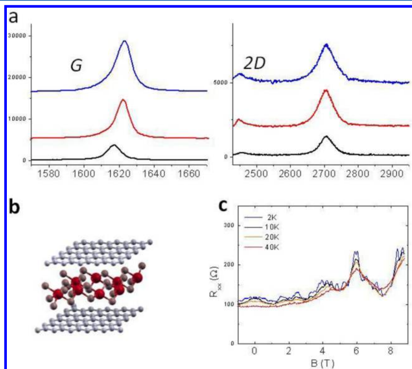
Figure 86. (a) Raman spectra of intercalated FLGs. (b) Atomic structural model; carbon atoms are shown as gray spheres, iron atoms as red, and chlorine atoms as brown. (c) Transport measurements of an intercalated bilayer device; Shubnikov-de Haas (SdH) oscillations seen in R_{xx}(B) are recorded at temperatures 2, 10, 20, and 40 K. Reprinted with permission from ref 396. Copyright 2011 American Chemical Society.
