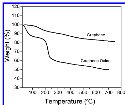
Figure 55. Thermal gravimetric analysis (TGA) plots of GO and chemically converted graphene nanoplatelets obtained using microwave irradiation. Reprinted with permission from ref 329. Copyright 2009 Royal Society of Chemistry.
