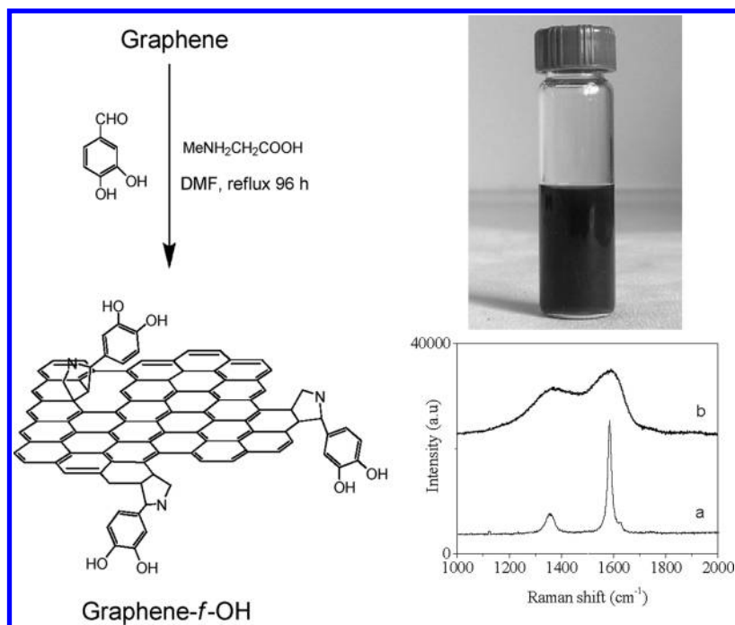
Figure 5. (left) Schematic representation of the 1,3 dipolar cycloaddition of azomethine ylide on graphene. (top, right) Dispersion of functionalized graphene nanoplatelets in ethanol. (bottom, right) Raman spectra of (a) pristine graphene and (b) pyrrolidine functionalized graphene. Reprinted with permission from ref 79. Copyright 2010 Royal Society of Chemistry.
