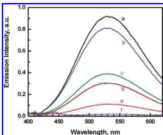
Figure 68. Emission spectra of a 1 mM ZnO suspension at different GO concentrations: (a) 0, (b) 0.035, (c) 0.09, (d) 0.14, (e) 0.20, and (f) 0.24 mg/mL. Reprinted with permission from ref 356. Copyright 2009 American Chemical Society.
