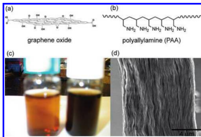
Figure 19. Schematic representation of (a) GO and (b) PAA. (c) Photograph of an aqueous colloidal dispersion of GO (left) and PAA-GO (right). (d) SEM image of the cross section of a PAA-GO paper sample. Reprinted with permission from ref 113. Copyright 2009 American Chemical Society.
