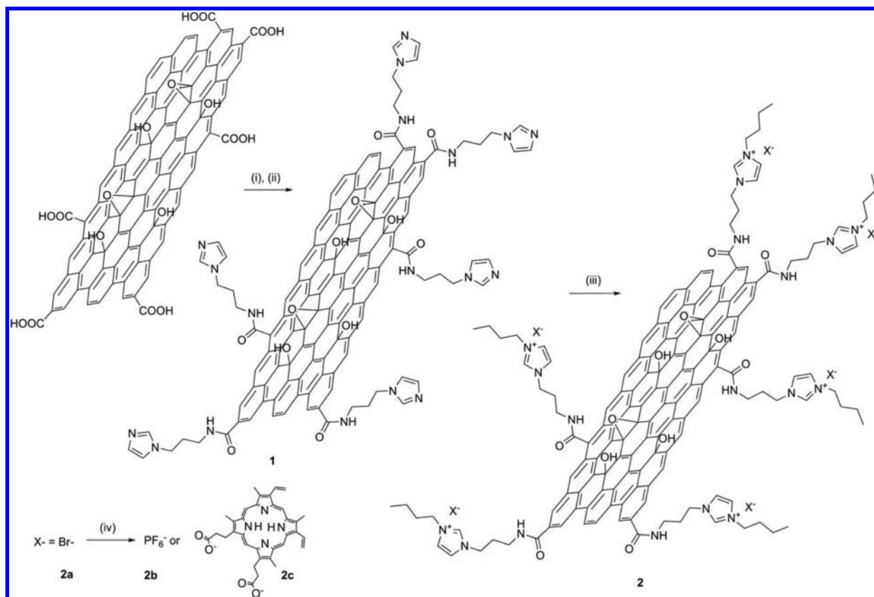
Figure 23. Preparation of imidazolium-modified GO hybrid materials and anion-exchange reactions: (i) (\text{COCl})_2 , 80 °C, 18 h; (ii) 1-(3-aminopropyl)imidazole, 100 °C, 18 h; (iii) 1-bromobutane, 90 °C, 18 h; (iv) \text{H}_2\text{O} , \text{NaPF}_6 or protoporphyrin IX disodium salt, 25 °C, 18 h. Reprinted with permission from ref 136. Copyright 2010 Elsevier.
