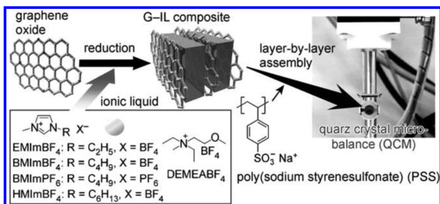
Figure 93. Schematic illustration of the preparation of a GO/ionic liquid multilayered composite and their LbL assembly on a quartz crystal microbalance (QCM). Reprinted with permission from ref 403. Copyright 2010 Wiley.
