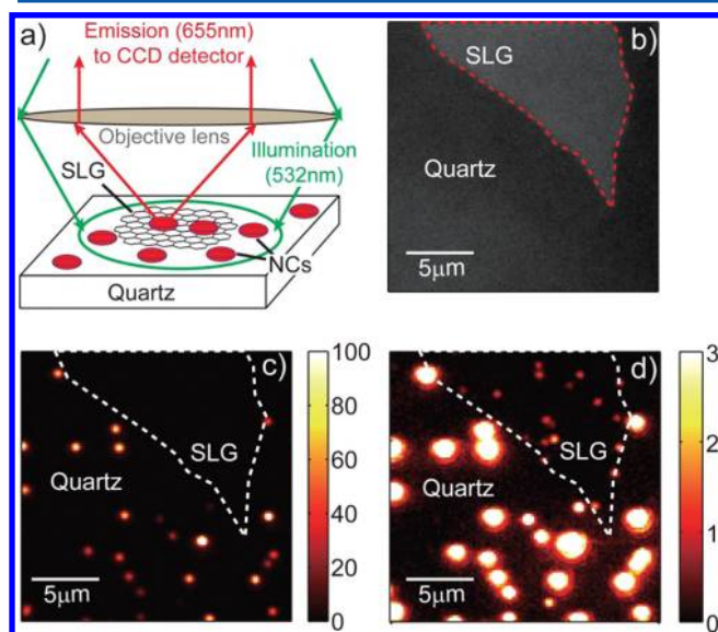
Figure 72. (a) Schematic representation of the experiment. (b) Optical reflectivity image in the emission range of the nanocrystals. (c, d) Wide-field fluorescence images of individual CdSe/ZnS nanocrystals in the region shown in panel b. Reprinted with permission from ref 369. Copyright 2010 American Chemical Society.
