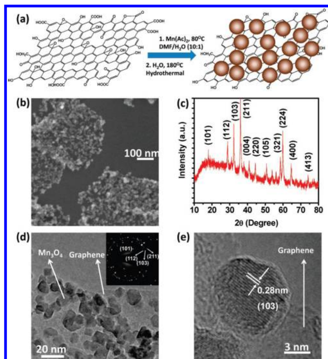
Figure 60. Mn 3 O 4 NPs grown on GO: (a) schematic two-step synthesis of Mn 3 O 4 /RGO, (b) SEM image of the Mn 3 O 4 /RGO composite, (c) XRD spectrum of Mn 3 O 4 /RGO, (d) TEM image of Mn 3 O 4 /RGO with inset showing the electron diffraction pattern of the Mn 3 O 4 NPs on RGO, and (e) high-resolution TEM image of an individual Mn 3 O 4 NP on RGO. Reprinted with permission from ref 340. Copyright 2010 American Chemical Society.
