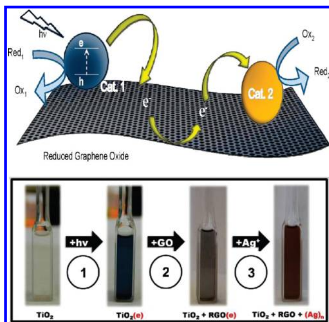
Figure 65. (top) RGO as a conducting pathway. (bottom) Photographs showing the color changes observed during stepwise transfer of electrons: (1) storage of electrons in TiO 2 by irradiation of the suspension with UV light; (2) addition of GO; the resulting gray color is due to the formation of RGO; (3) upon the addition of AgNO 3 , reduction of Ag + to Ag NPs (red color) by stored electrons in the RGO occurs. Reprinted with permission from ref 354. Copyright 2010 American Chemical Society.
