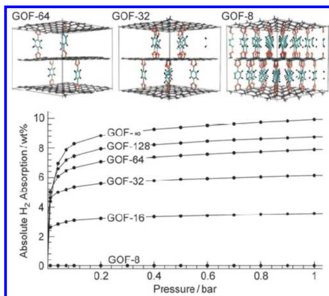
Figure 88. Grand canonical Monte Carlo simulations for ideal GOF- n structures with n graphene carbons per linker. The structures of three examples with n = 64, 32, and 8 are also shown. GOF materials are formed of layers of GO connected by benzenediboric acid pillars. Reprinted with permission from ref 399. Copyright 2010 Wiley.
