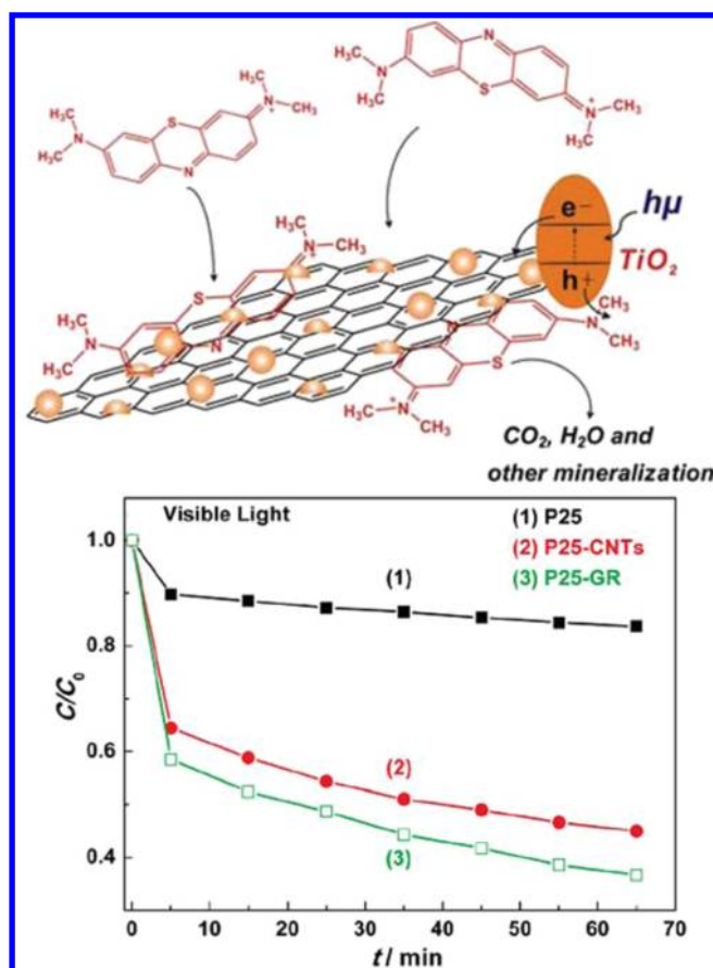
Figure 66. (top) Schematic representation of the photodegradation of methylene blue on the P25/GO composite and (bottom) photodegradation of methylene blue under visible light using (1) P25, (2) P25–carbon nanotubes, and (3) P25–RGO photocatalysts. Reprinted with permission from ref 352. Copyright 2010 American Chemical Society.
