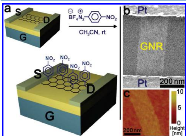
Figure 1. Chemical doping of graphene with 4-nitrophenyl groups: (a) schematic representation; (b) SEM image of a graphene nanoribbon between Pt electrodes; (c) AFM image of a fragment of a monolayer graphene. Reprinted with permission from ref 64. Copyright 2010 American Chemical Society.
