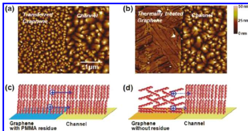
Figure 83. AFM images of pentacene films (50 nm) near the interface between SiO 2 : (a) untreated graphene electrodes and (b) thermally treated graphene electrodes. Schematic representations of the possible molecular packing orientations near the interface between SiO 2 and (c) untreated graphene electrodes or (d) thermally treated graphene electrodes. Reprinted with permission from ref 391b. Copyright 2011 Wiley.
