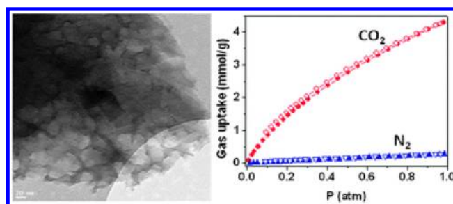
Figure 99. (left) TEM image of the polypyrrole graphene hybrid activated at 600 °C and (right) absorption selectivity of CO 2 gas over N 2 gas at 298 K. Reprinted with permission from ref 427. Copyright 2012 Royal Society of Chemistry.
