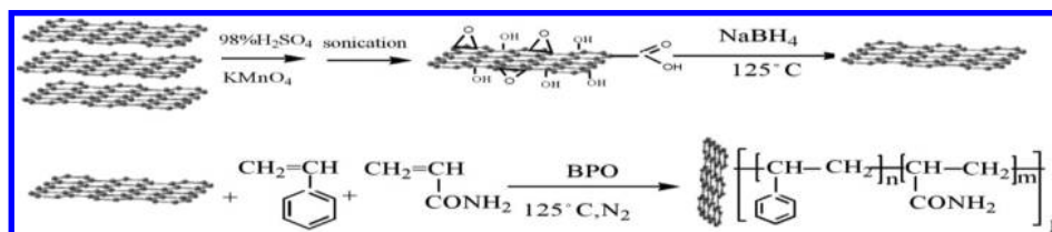
Figure 30. Schematic representation of covalent attachment of PS/PAM copolymer to RGO. Reprinted with permission from ref 153. Copyright 2009 Wiley.
