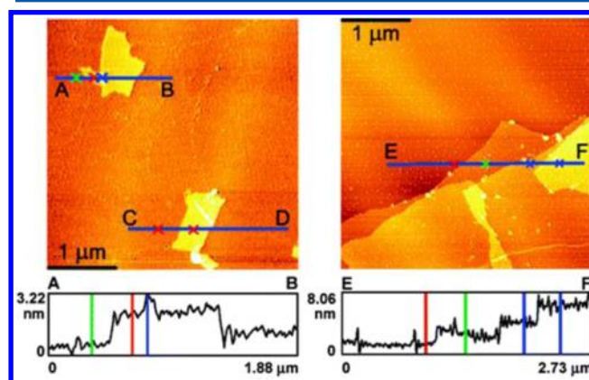
Figure 38. (left) Tapping mode AFM images of exfoliated GO and (right) PB^- functionalized graphene on mica. Reprinted with permission from ref 267. Copyright 2008 American Chemical Society.
