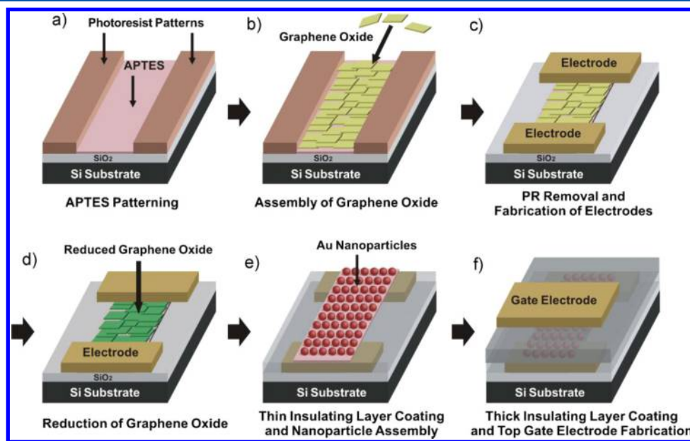
Figure 53. Schematic representation of the fabrication process of RGO-based memory devices using Au NPs. Reprinted with permission from ref 320. Copyright 2010 Wiley.
