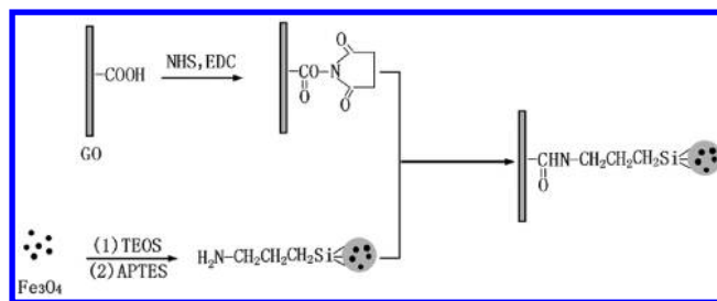
Figure 71. Schematic representation of the GO/Fe 3 O 4 NPs. Reprinted with permission from ref 363. Copyright 2010 Elsevier.
