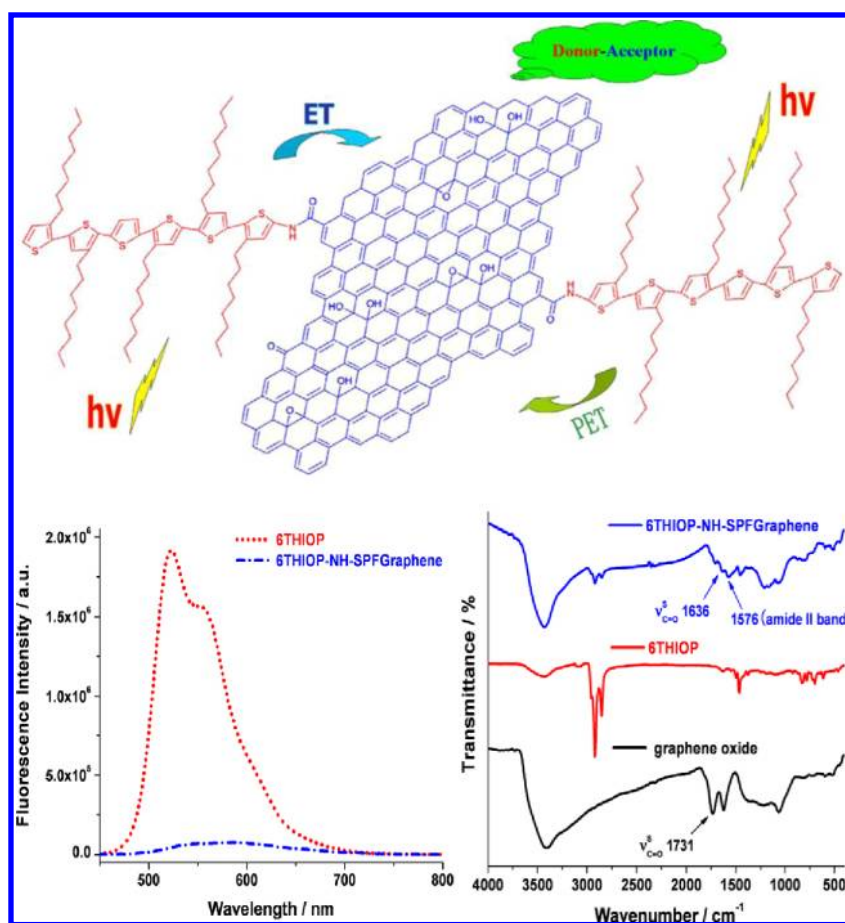
Figure 12. (top) Structure of oligothiophene functionalized GO. (bottom, left) Fluorescence spectra of oligothiophene–GO compared with that of pure oligothiophene. (bottom, right) FTIR spectra of GO, oligothiophene (6Thiop), and the functionalized GO (6Thiop-NH-SPFGraphene). Reprinted with permission from ref 103. Copyright 2009 Elsevier.
