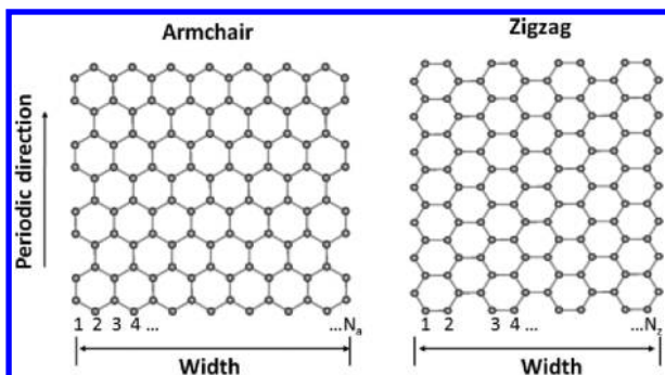
Figure 94. Structure of armchair and zigzag nanoribbons.
