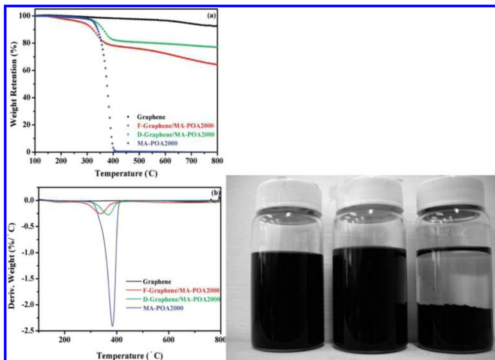
Figure 29. (a) Thermogravimetric curves and (b) corresponding derivative curves of the starting materials and the derivatives. Photograph showing the dispersion of graphene, F-graphene/MA-POA2000 and D-graphene/MA-POA2000 in THF (from right to left). Reprinted with permission from ref 152. Copyright 2010 American Chemical Society.
