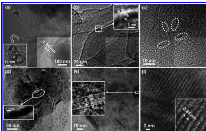
Figure 45. HRTEM micrographs of (a) neat ILFG showing the crumpled sheet like texture (inset on right-hand side shows the thickness of the nanosheet), (b) neat RGO with the inset showing a blown up view of a fold on the nanoplatelet, (c) the PEDOT–RGO nanocomposite; the ellipses encircle the streak like structures typical of RGO and are surrounded by the amorphous polymer, (d) PEDOT–ILFG nanocomposite, the elongated shapes (as in the inset) are characteristic of ILFG, (e) coexisting crystalline and amorphous phases in PEDOT–ILFG (inset is a magnified view of a quasi-ordered arrangement of lattice fringes), and (f) a relatively defect free crystallite of ILFG in PEDOT–ILFG (the inset shows the fringe separation of 0.85 nm). Reprinted with permission from ref 287. Copyright 2011 American Chemical Society.
