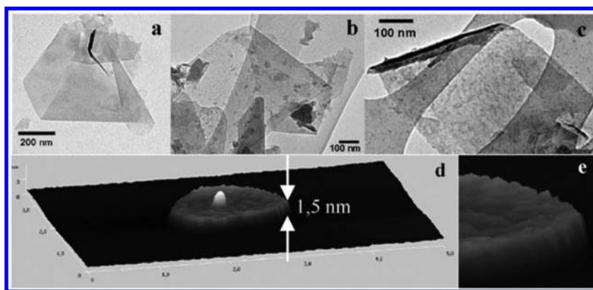
Figure 6. (top) Characteristic TEM and (bottom) AFM images of the graphene- f -OH isolated from an ethanol dispersion. Reprinted with permission from ref 15. Copyright 2009 Nature Publishing Group.
