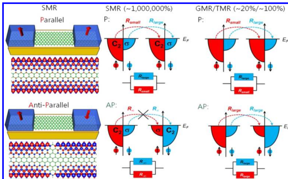
Figure 95. Schematic ZGNR-based spin-valve device (left) with parallel and antiparallel spin configurations and the corresponding spin-magnetization density isosurfaces. The blue boxes represent ferromagnetic electrodes to control spin polarization of the ZGNR device and the red arrows indicate the directions of spin configurations. In the isosurfaces, red/blue color denotes up/down spin, and a ZGNR skeleton is drawn in green color. Spin-transfer paths (right) from the left to right density of states of the ferromagnetic leads for parallel (P) and antiparallel (AP) spin configurations in a ZGNR spin-valve device are compared with those in a conventional spin-valve device. Reprinted with permission from refs 29 and 409. Copyright 2008 Nature Publishing group and Copyright 2010 American Chemical Society, respectively.
