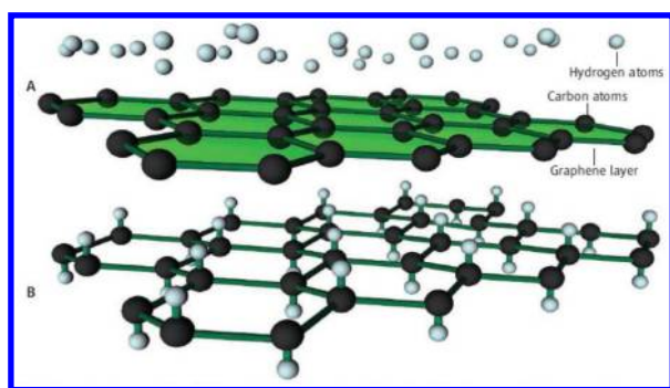
Figure 31. Graphene layer (in green) that is attacked by cold plasma hydrogen atoms to produce graphane. Reprinted with permission from ref 159. Copyright 2009 American Association for the Advancement of Science.
