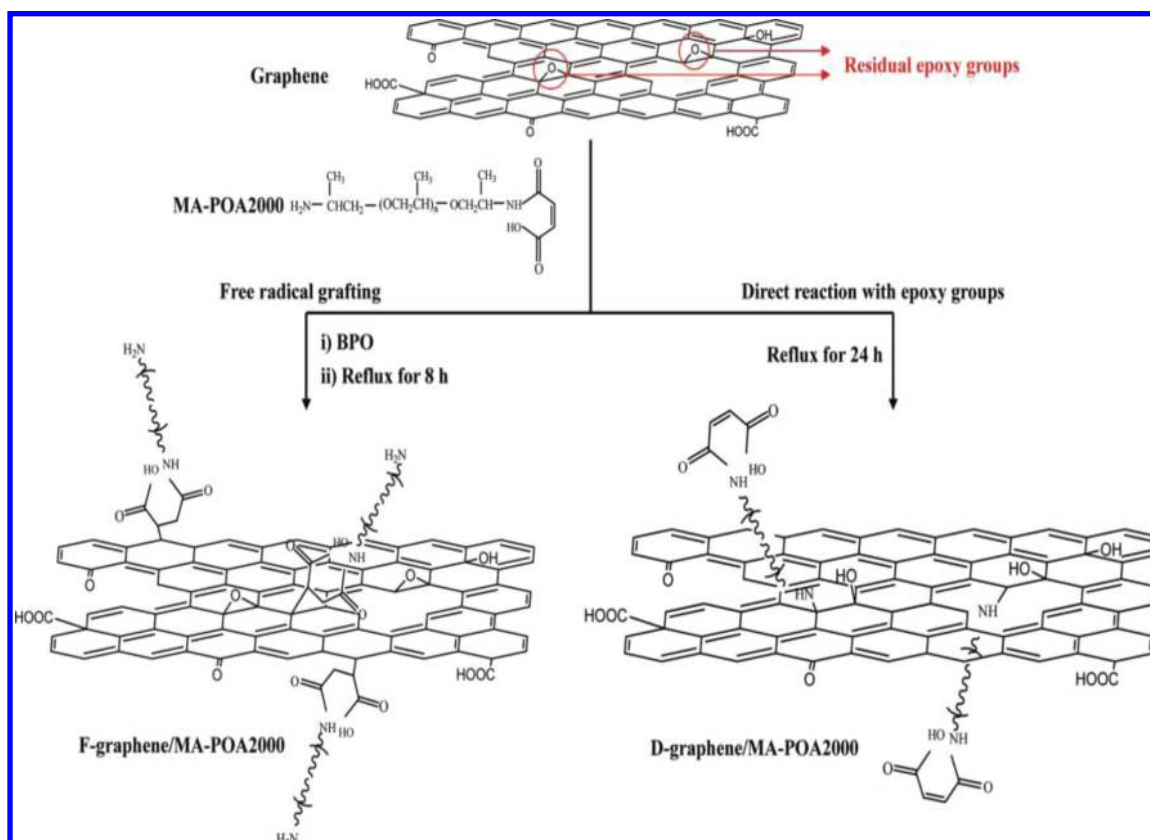
Figure 28. Two different grafting methods from the same organic molecule. Reprinted with permission from ref 152. Copyright 2010 American Chemical Society.
