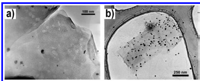
Figure 52. TEM images of the RGO–Au composite on a holey carbon grid: (a) sequential reduction sample; (b) simultaneous reduction sample. Reprinted with permission from ref 319. Copyright 2010 American Chemical Society.
