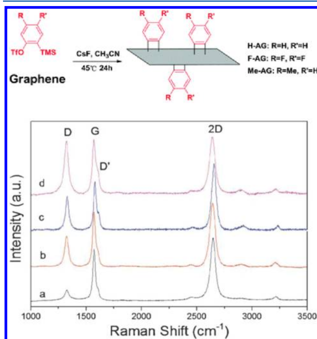
Figure 10. (top) Aryne cycloaddition to graphene sheets. (bottom) Raman spectra of (a) pristine and (d) functionalized graphene nanoplatelets by aryne, (c) methylated aryne, and (b) fluorinated aryne. Reprinted with permission from ref 88. Copyright 2010 Royal Society of Chemistry.
