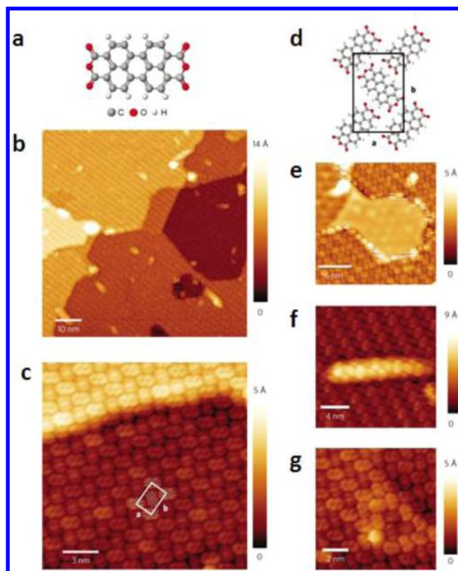
Figure 42. (a) Molecular structure of PTCDA. (b) Monolayer coverage of PTCDA on epitaxial graphene. (c) Molecular-resolution STM image of the PTCDA monolayer. (d) PTCDA herringbone unit cell, with the lattice vectors ( a and b ). (e) PTCDA surrounding a step edge where the graphene sheet is not continuous. (f) PTCDA continuously covers a graphene-subsurface nanotube defect. (g) A bright protrusion that does not disrupt the PTCDA monolayer and that is potentially attributed to a 6-fold scattering-center defect ( V_s = -2.0 V, I = 0.05 nA for all five STM images). Reprinted with permission from ref 38. Copyright 2009 Nature Publishing Group.
