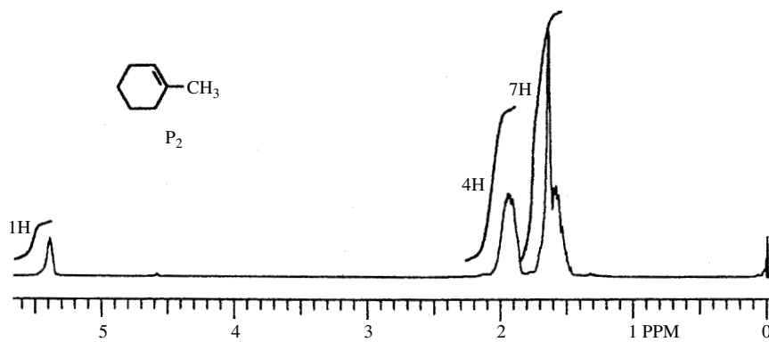
Figure 11.26 1-Methylcyclohexene.
